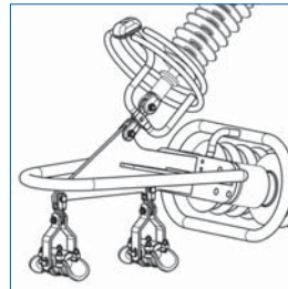
Yoke for the insulating crossarm
