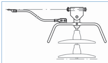
Shunt for high short circuit currents
