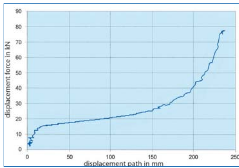
Example of the operating line of the displacement element
