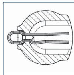
Security split pin inserted in the socket eye
