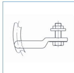
Arcing device for a big string displacement
