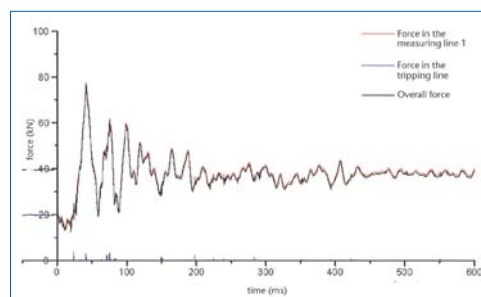
Chronological sequence of tensile force in the intact string
