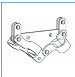
Displacement yoke for suspension strings
