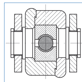
Cross section of a double wedge tension clamp
