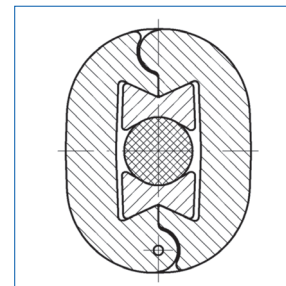
Cross section of a wedge tension clamp
