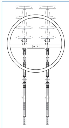
400 kV tension tower: 2 systems for a quadruple bundle
