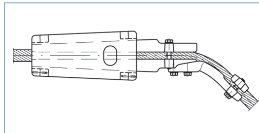
Wedge tension clamp with jumper connection
