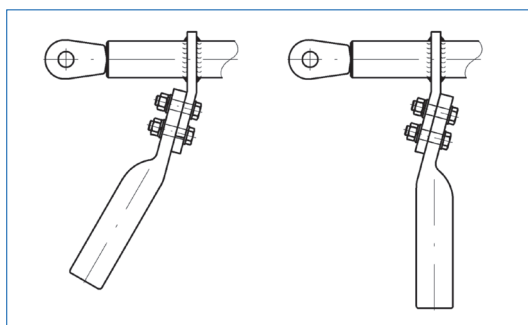
Possible connection variants of the jumper
