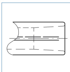
Taper of compression dead end clamps - standard design
