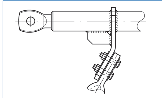
Compression dead end clamp with an increased retaining force for the loop
