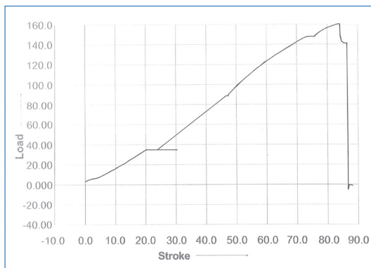
Typical force-way chart for a compression dead end clamp
